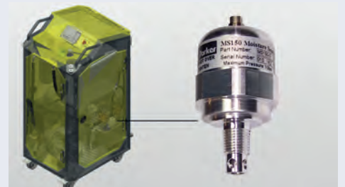
Fig4. A Parker MS150 moisture sensor provides continuous monitoring of moisture content in the oil to determine moisture levels and operation.
